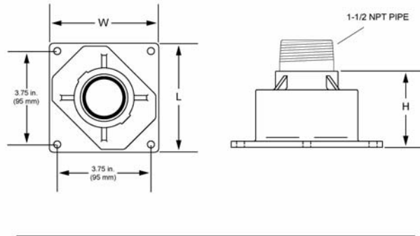
SVFT-PR-P Dimensions
