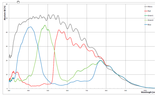
Quantum Efficiency Curve for Mono Sensor
