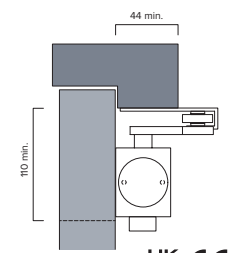
Fig.66 Parallel arm push side mount
