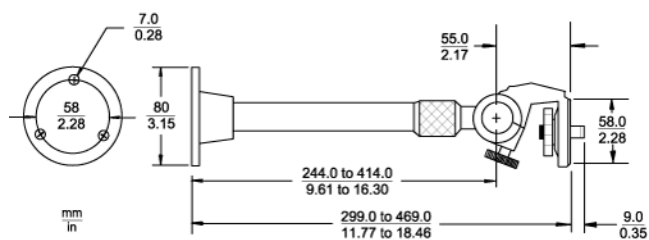
TC9202 Indoor Camera Mount
