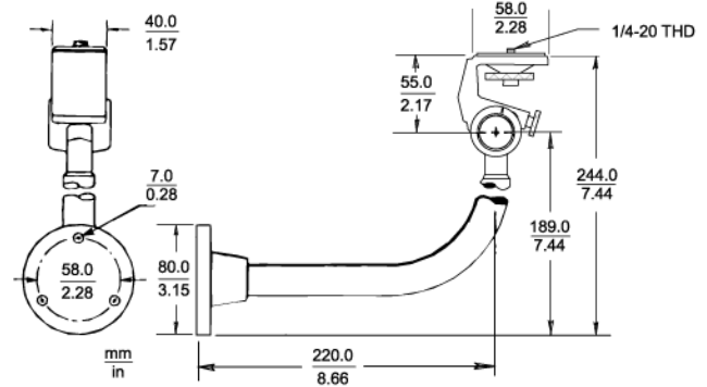
TC9203 Indoor Camera Mount
