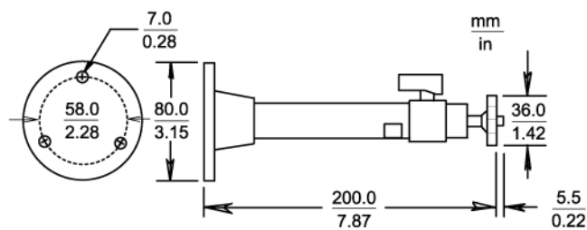
TC9201 Indoor Camera Mount
