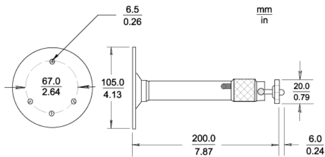
TC9200 Indoor Camera Mount
