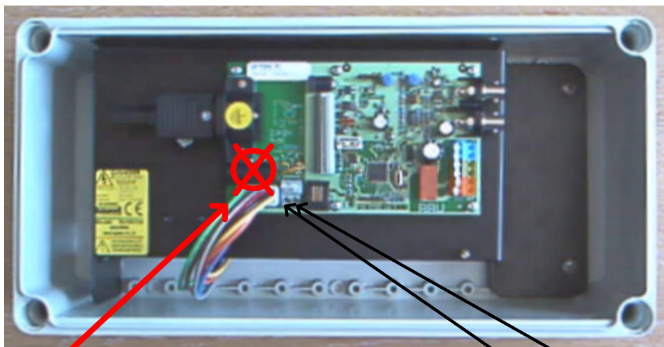
Fig 10. RX100/24 iss. 6 pcb Connection details when operating from a 24Vac supply.
