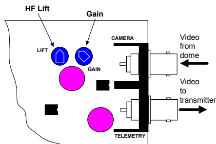
Fig. 3 Launch Amplifier
