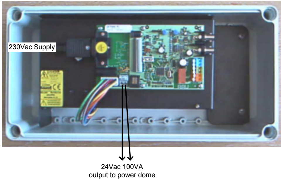
Fig 9. RX100/24 iss. 6 pcb Connection details when operating from a 230Vac supply.
