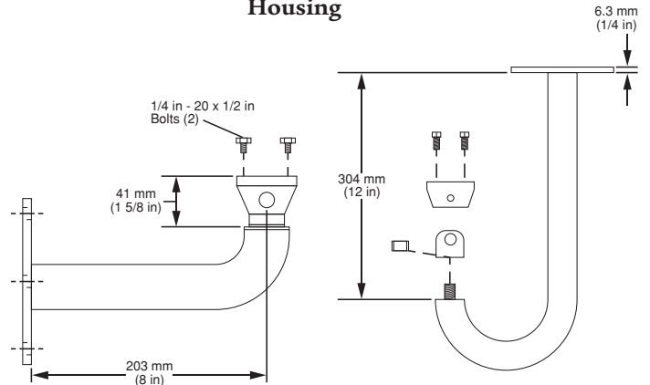
Wall Mount Side View ADCHMTWALL
